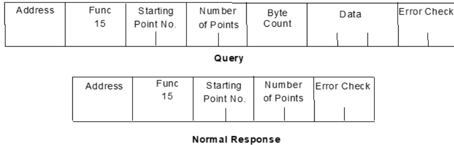
Figure 70: RTU Force Multiple Outputs Message Format
