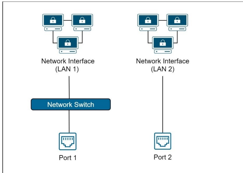
Figure 37: Dual-LAN Mode
