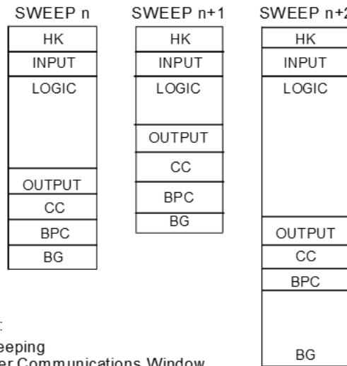
Figure 48: Typical Sweeps in Normal Sweep Mode
