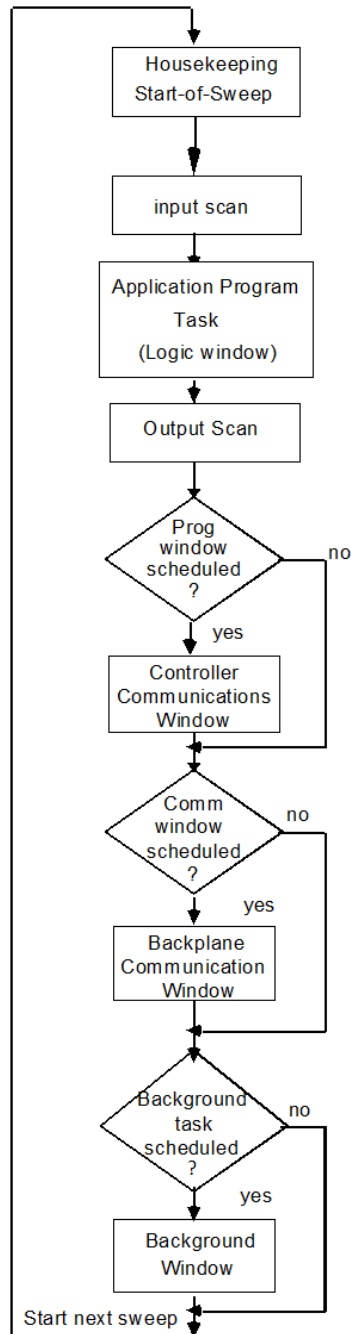
Figure 47: Major Phases of a Typical CPU Sweep
