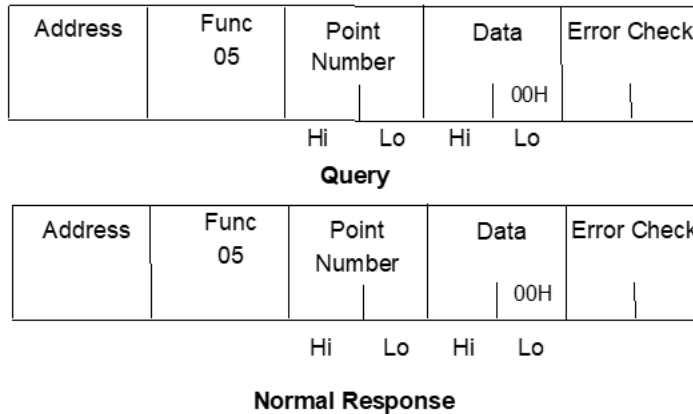
Figure 66: RTU Force Single Output Message Format
