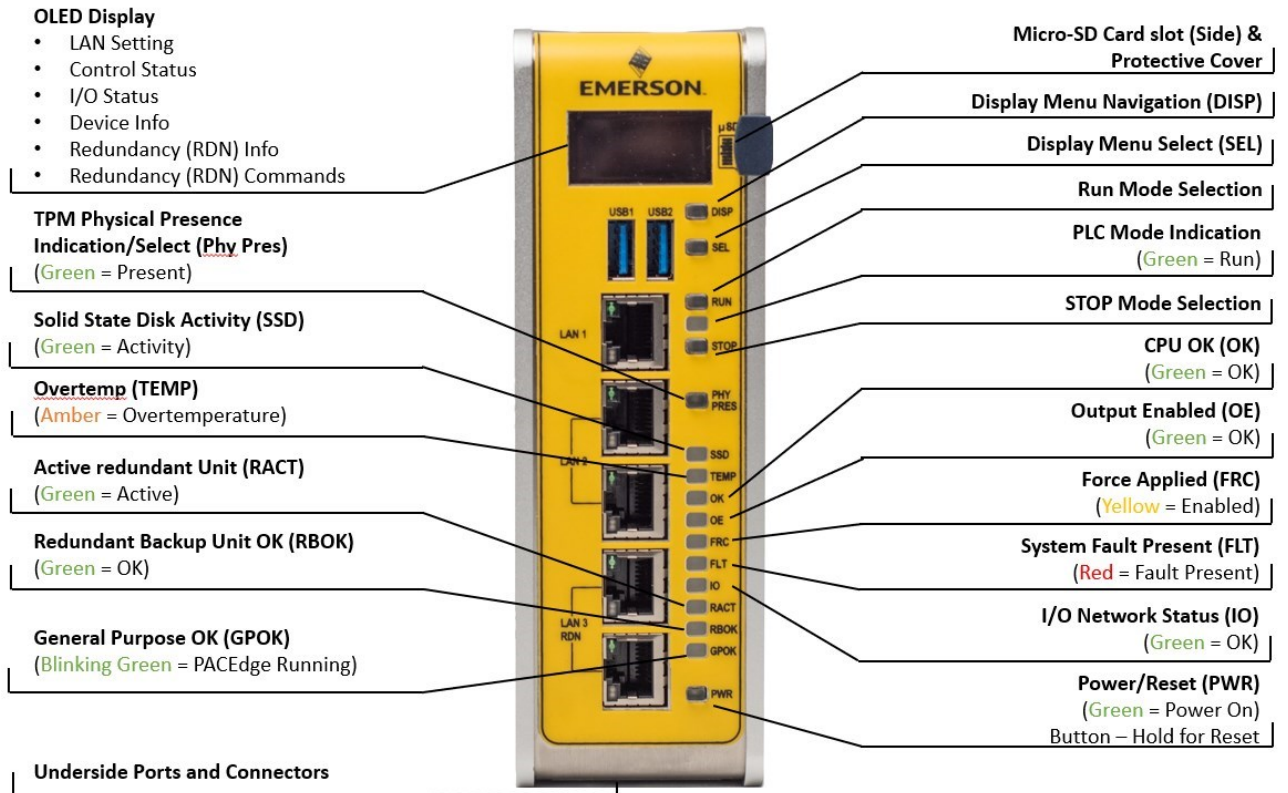
Figure 4: CPS400 Front View and Features
