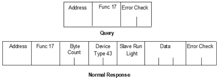
Figure 72: RTU Report Device Type Message Format
