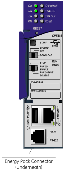
Figure 16: External Features of CPE302/CPE305-Axxx
